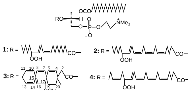
Scheme 1. Phosphatidylcholine hydroperoxides.
